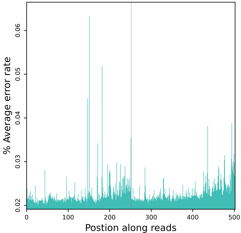
Error rate distribution along reads (R10612)
